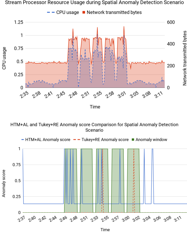
Fig. 2: Spatial anomalies are injected by increasing the workload for the stream processors as represented by the five bursts in the first plot. The next plot shows the anomaly scores produced by both HTM+AL and Tukey+RE models during the anomalous periods.
