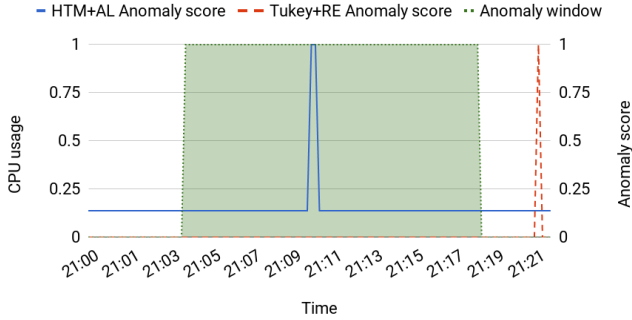
Fig. 4: Regular workload consists of high workload followed by low workload. Temporal anomalies were injected where high workload was observed but low workload was expected, as shown in the first plot. The next plot shows the anomaly scores produced by both HTM+AL and Tukey+RE models during the anomalous period.
