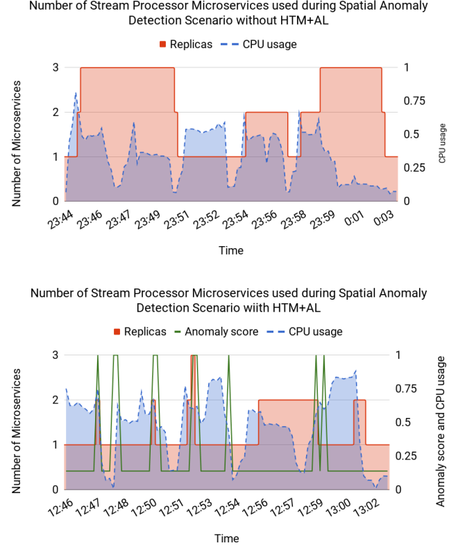
Fig. 3: Without HTM+AL, the AMS scaled microservices to handle the unnecessary workload produced by spatial anomalies, as shown in the first plot. In the next plot, the AMS was able to detect most of the spatial anomalies with HTM+AL and minimized the economic damage by 38.12%.
